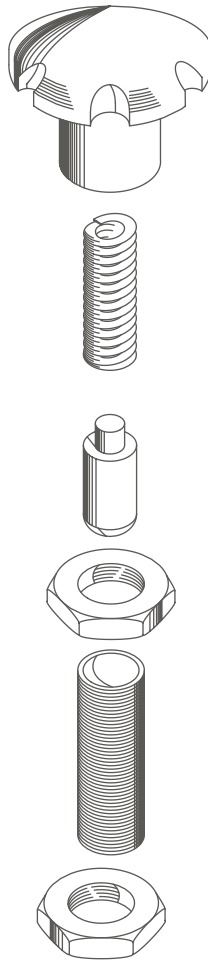
Hand knob assembly part number 7800127
